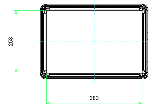
C-C (1:6.5)
